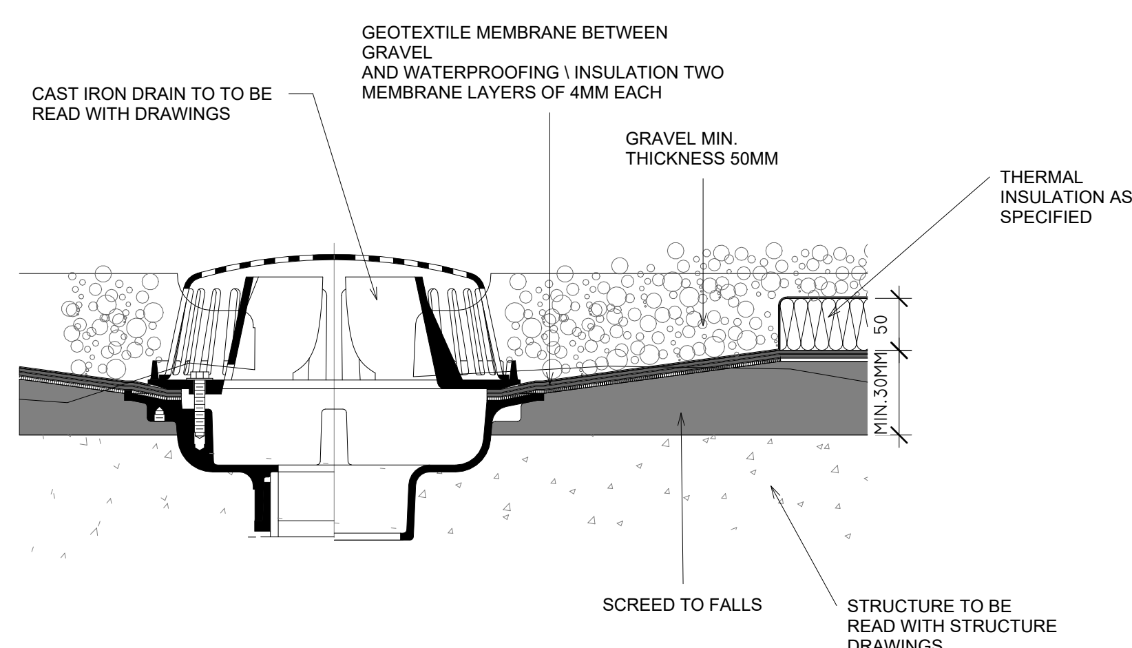
18 TYPICAL ROOF DRAINAGE DETAIL 1 : 5
