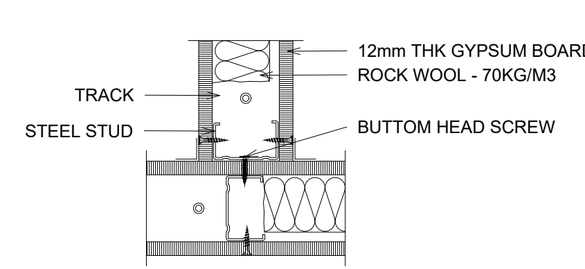
5 TYP. T-JUNCTION JOINT 1 : 5
