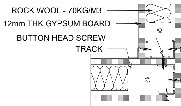
1 TYP. CORNER JOINT 1 : 5
