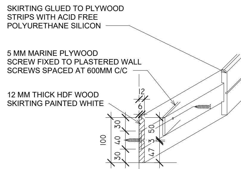
8 TYP. SKIRTING ASSEMBLY DETAIL 1 : 5
