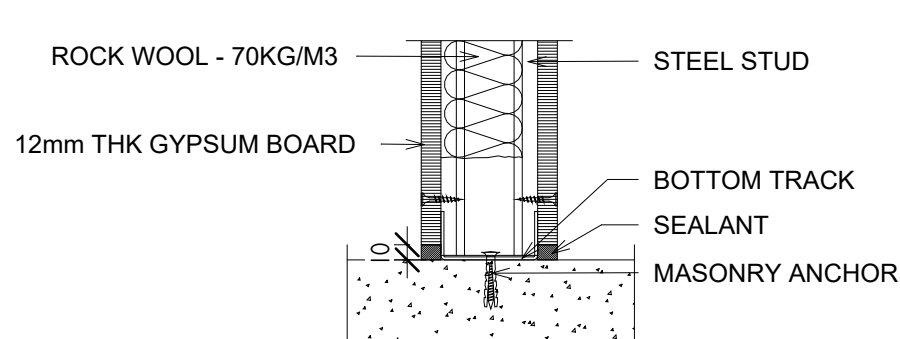
2 TYP. CONNECTION TO FLOOR 1 : 5
