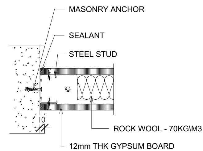
3 TYP. CONNECTION TO WALL 1 : 5
