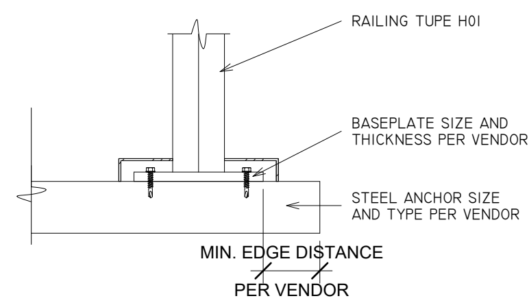
12 HANDRAIL DETAILS 1 : 5
