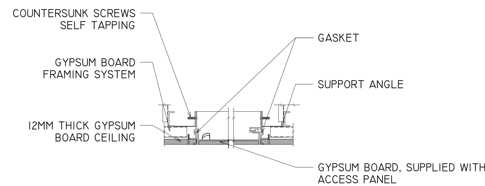
14 TYP. HINGED ACCESS PANEL SECTION 1 : 5
