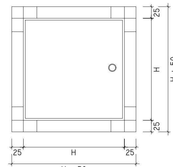
13 TYP. HINGED ACCESS PANEL PLAN 1 : 5
