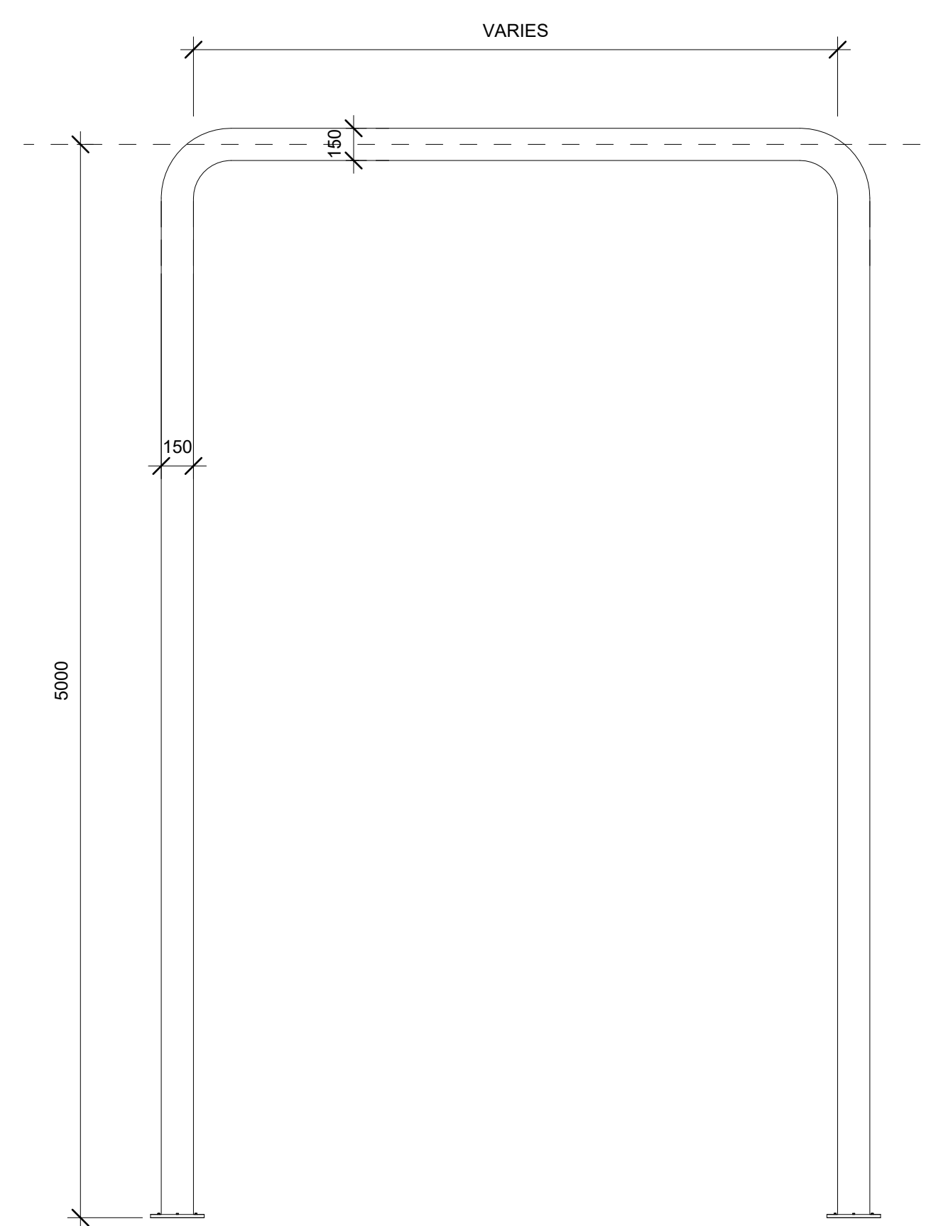
19 OVERHEAD SAFETY BARRIER (VENDOR) 1 : 25
