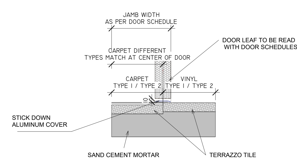
11 D-CARPET VINYL DETAIL 1 : 5
