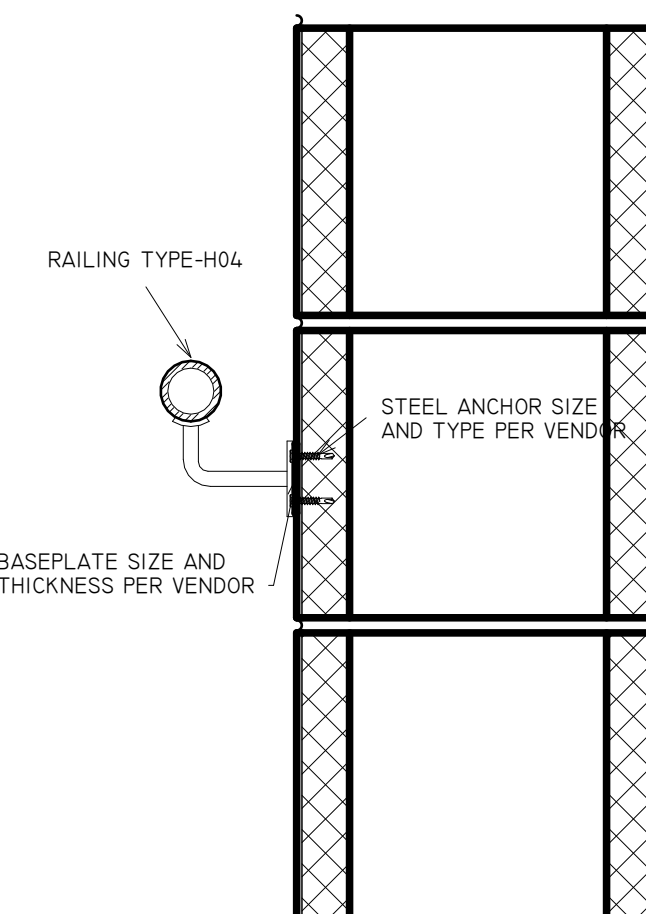
17 TYP. WALL MOUNTED HANDRAIL DETAILS 1 : 5
